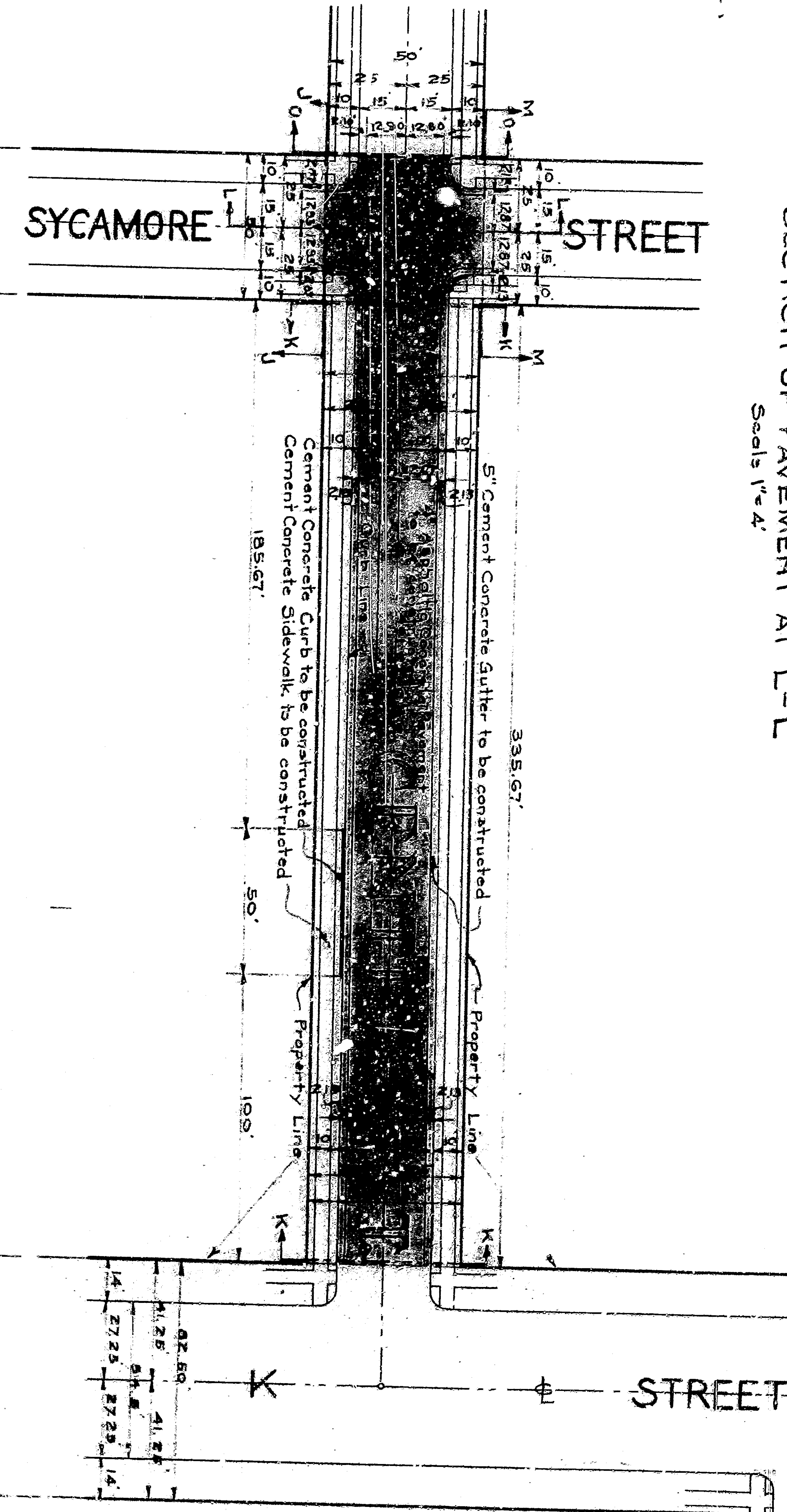
PLAN Scale 1" = 4'
